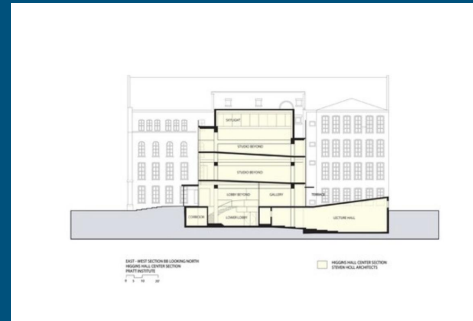
Partial section
