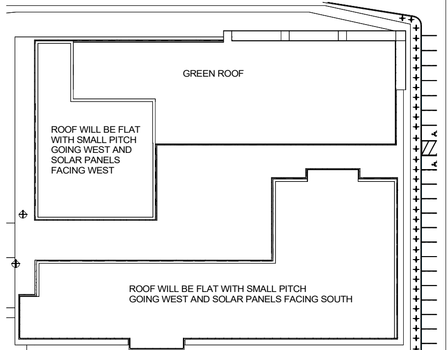
① ROOF PLAN AP
