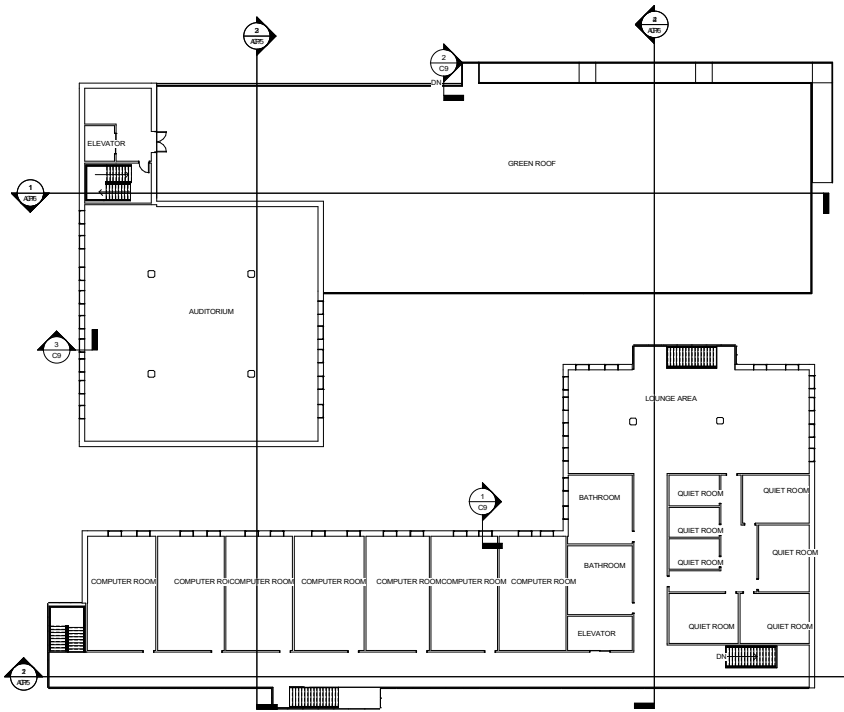
② SECOND FLOOR AP 1/16" = 1'-0"
