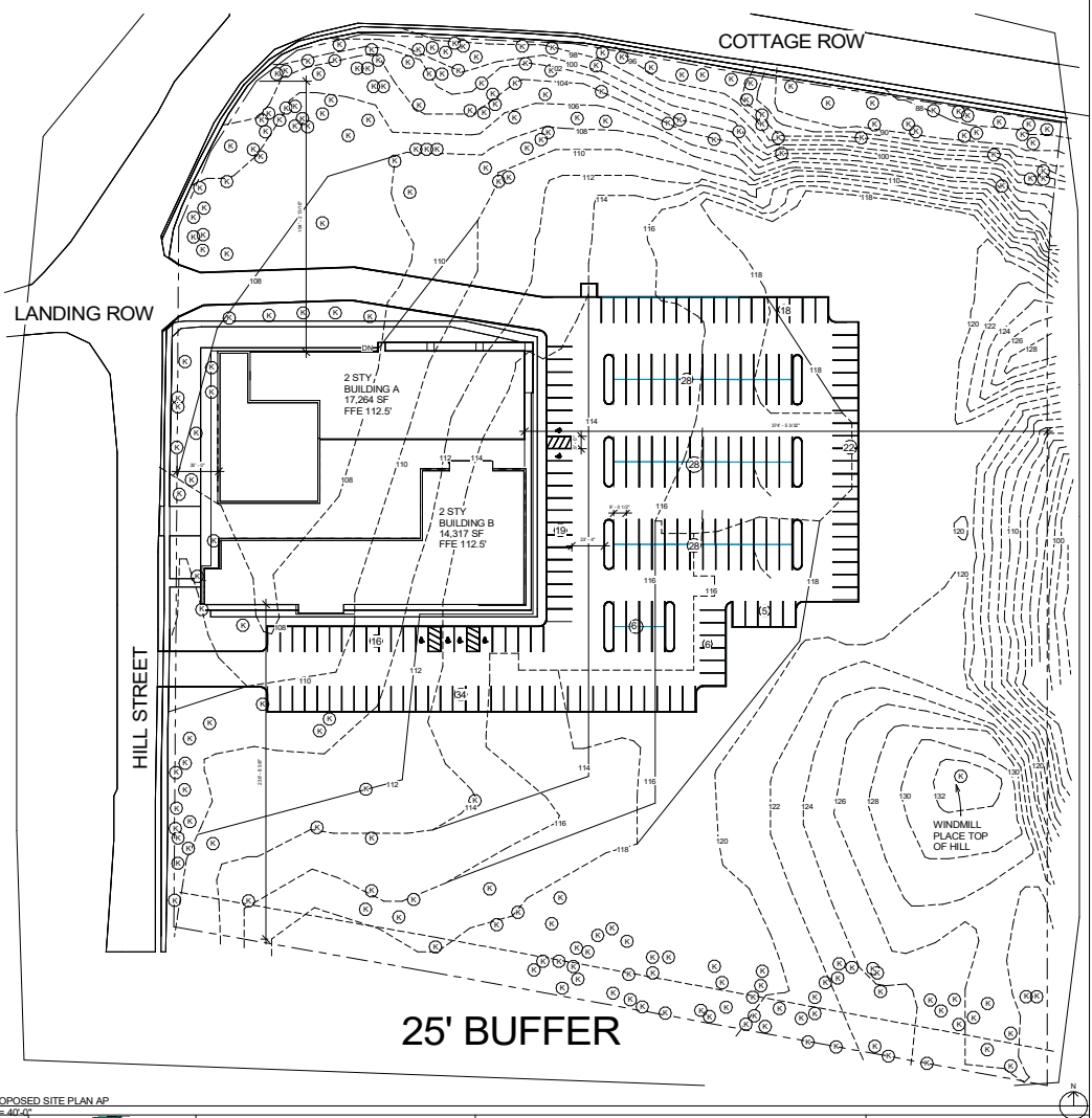
PROPOSED SITE PLAN AP 1" = 40' AT
