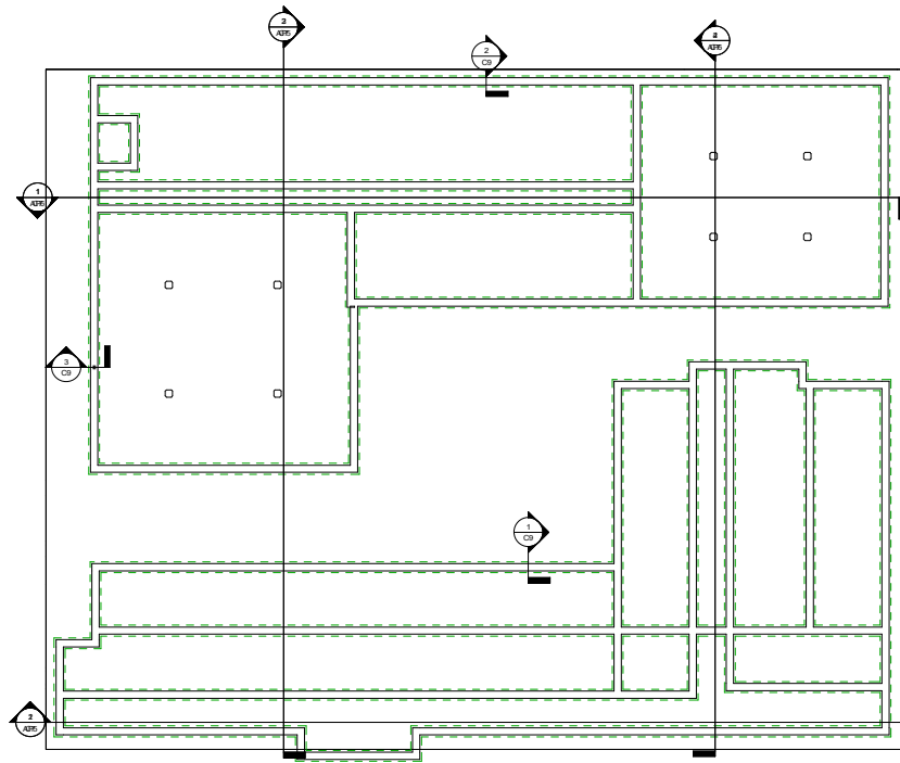
① FOUNDATION PLAN AP 1/16" = 1'-0"
