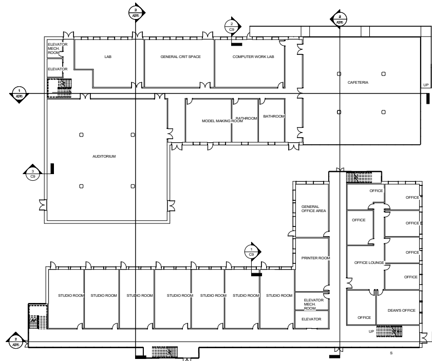
③ FIRST FLOOR PLANS AP 1/16" = 1'-0"
